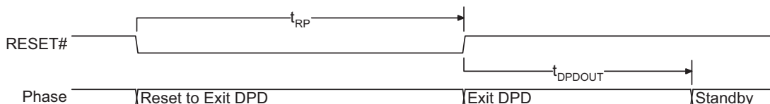
Figure 10.3 Deep Power Down RESET# Exit Timing
