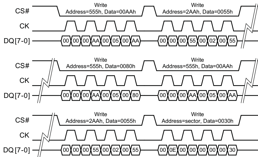
Figure 4.4 Write Transaction Usage Example: Erase Operation Command Sequence
