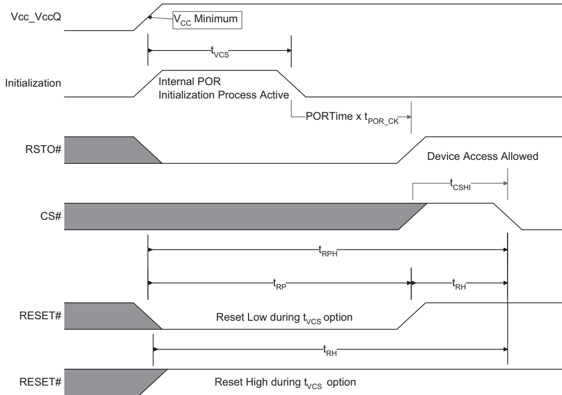
Figure 11.2 Power On Reset Signal Diagram
