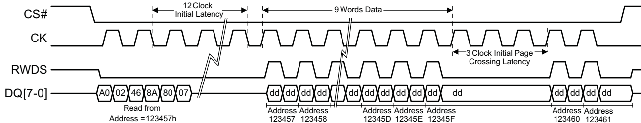
Figure 4.2 Read Transaction Crossing a Page Boundary
