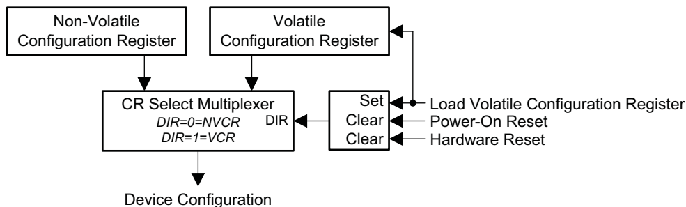
Figure 6.5 Configuration Control
