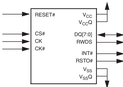
Figure 3.1 HyperFlash Interface
