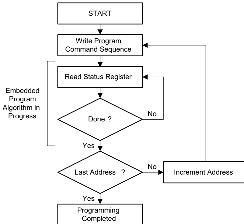
Figure 6.1 Word Program Operation
