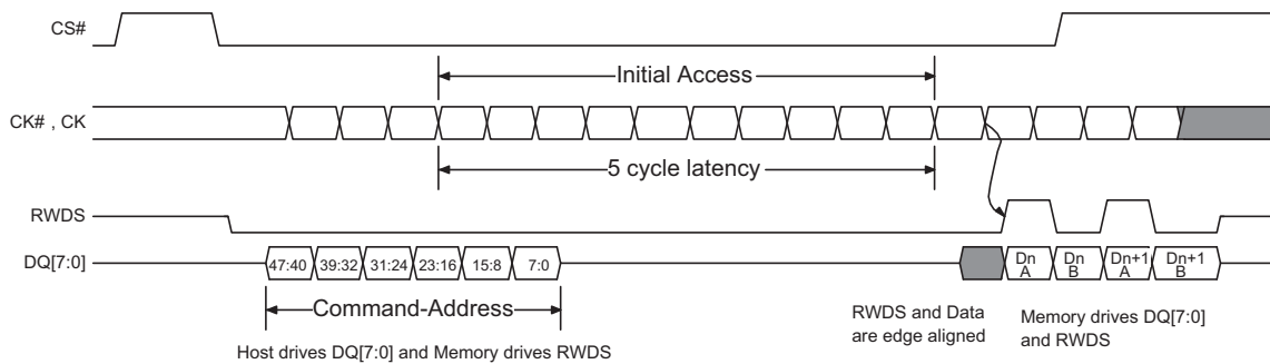
Figure 4.1 Read Operation
