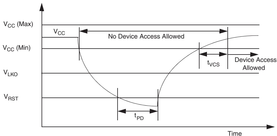
Figure 11.1 Power-Down or Voltage Drop
