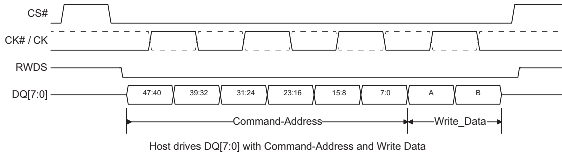
Figure 4.3 Write Operation
