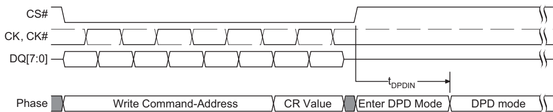
Figure 10.1 Deep Power Down Entry Timing
