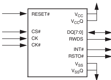
Figure 2.1 HyperFlash Interface
