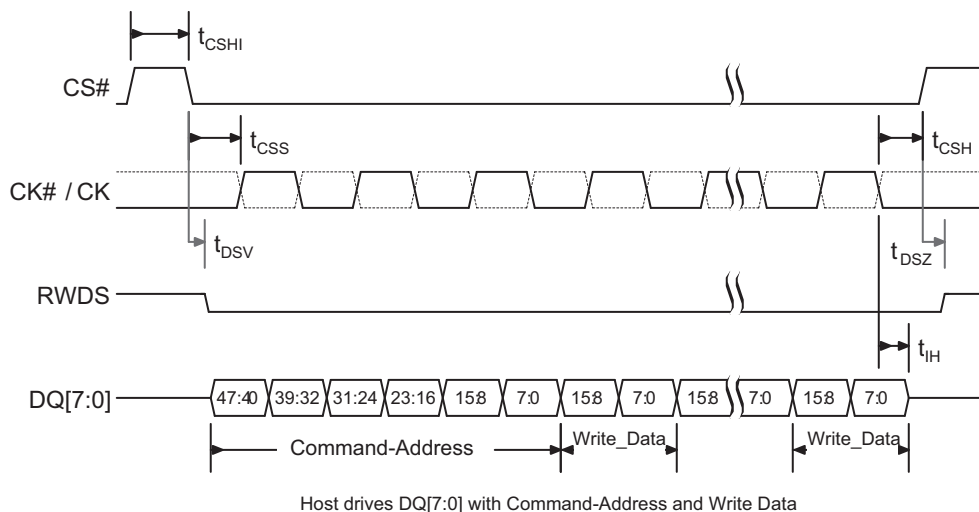
Figure 12.1 Burst Write During Load of Multiple Words During a Word Program Command Timing Diagram
