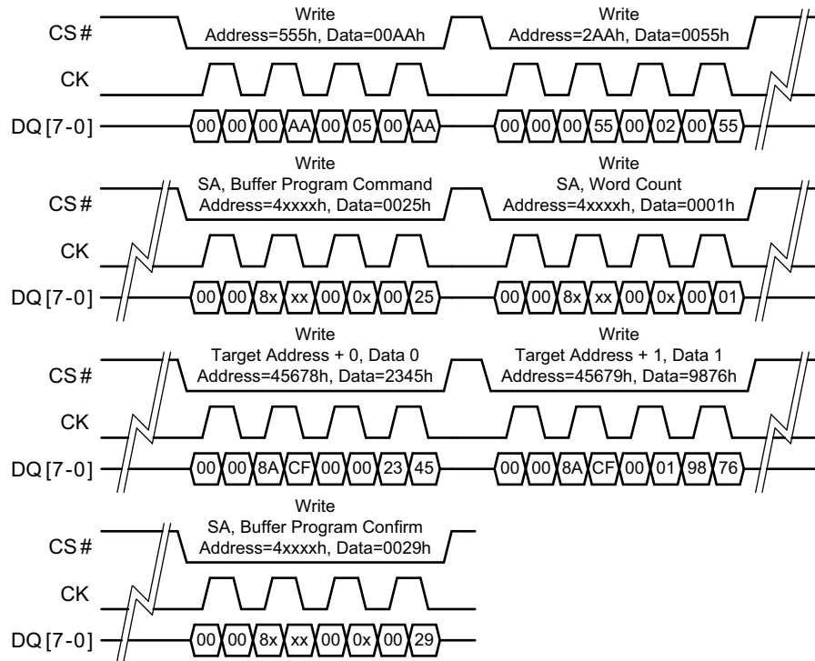
Figure 4.5 Write Transaction Usage Example: Write Buffer Program Command Sequence
