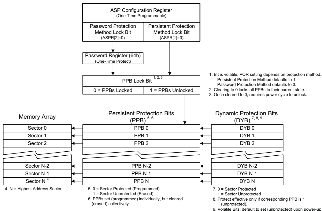
Figure 6.7 Advanced Sector Protection Overview
