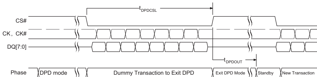
Figure 10.2 Deep Power Down CS# Exit Timing
