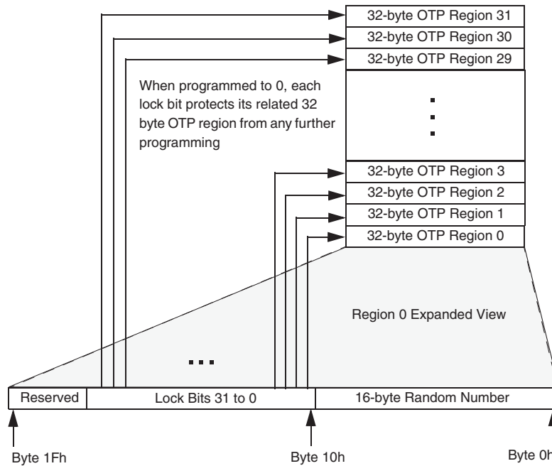
Figure 6.6 SSR Address Space
