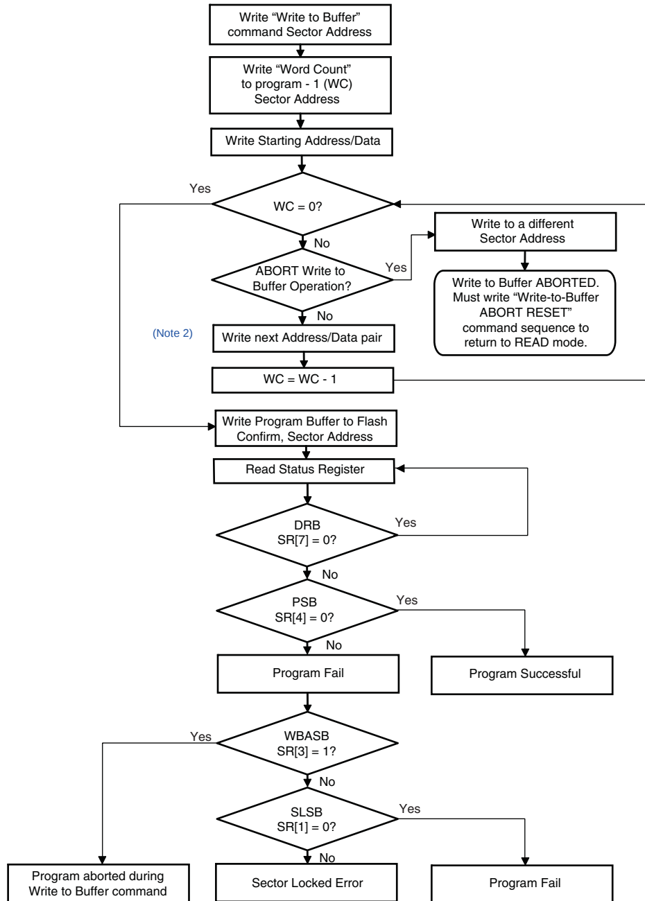
Figure 6.2 Write Buffer Programming Operation with Status Register
