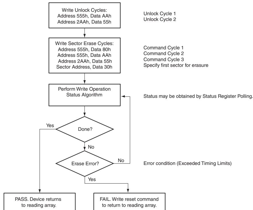
Figure 6.4 Sector Erase Operation
