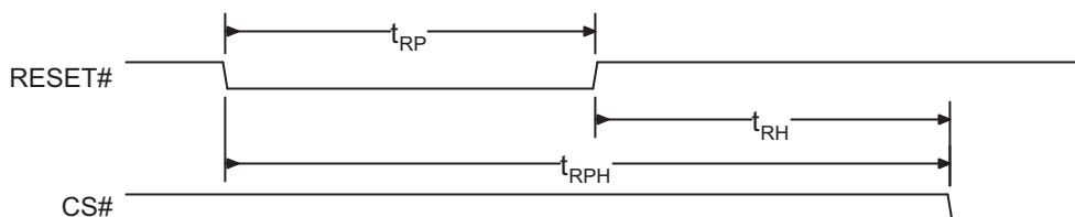
Figure 11.3 Hardware Reset Timing Diagram
