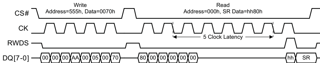
Figure 4.6 Status Read Transaction Example
