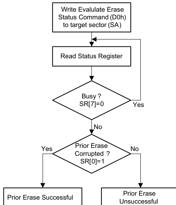
Figure 6.3 Evaluate Erase Status Software Sequence
